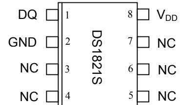
8-pin 208-mil SOIC (DS1821S)
